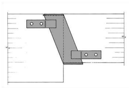
FIGURE 9A—TYPICAL INSTALLATION OF A THC HANGER
