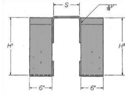
FIGURE 8B—THGLS HANGER
