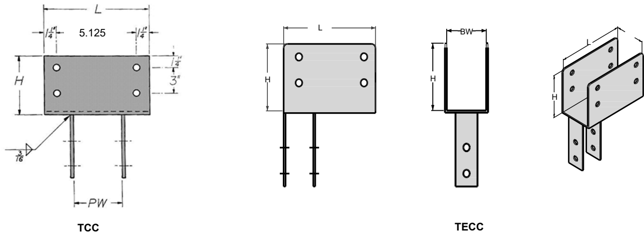
FIGURE 1—TYPICAL TCC and TECC COLUMN CAP CONNECTORS
