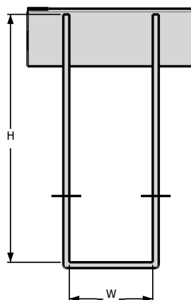
FIGURE 5—TYPICAL TXD SERIES HANGER
