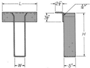
FIGURE 6A—TYPICAL TGLT SERIES HANGER L
