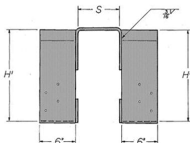
FIGURE 8B—THGLS HANGER
