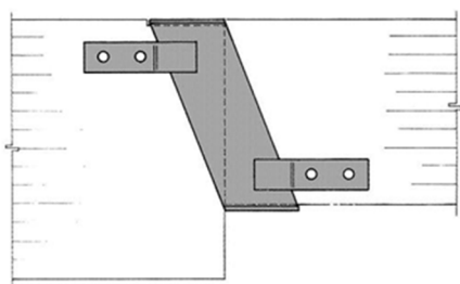
FIGURE 9A—TYPICAL INSTALLATION OF A THC HANGER
