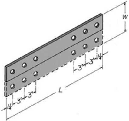
Figure 10B—DRAWING OF THE THST STRAP
