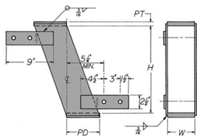
FIGURE 9B—TYPICAL THC HANGER
