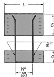
FIGURE 8C—TYPICAL THGLS HANGER
