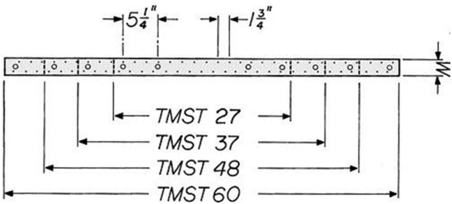
FIGURE 10D—DRAWING SHOWING THE RELATIVE LENGTHS OF THE TMST STRAPS (TMST72 similar; TSI similar, but without bolt holes)
