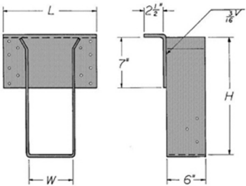
FIGURE 6C—TYPICAL THGLT SERIES HANGER
