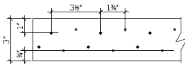
FIGURE 10E—DRAWING OF THE TCMST12 AND TCMST14 STRAPS
