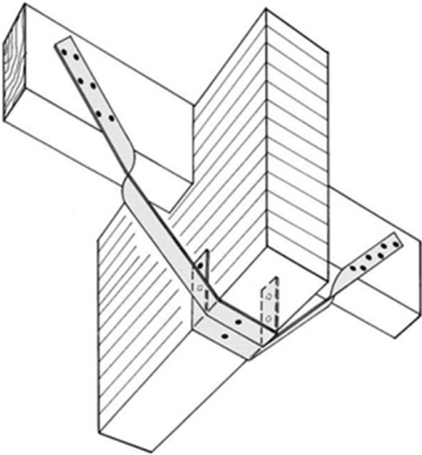
FIGURE 3—TYPICAL TVB KNEE BRACE INSTALLATION
