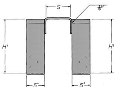
FIGURE 8A—TGLS HANGER
