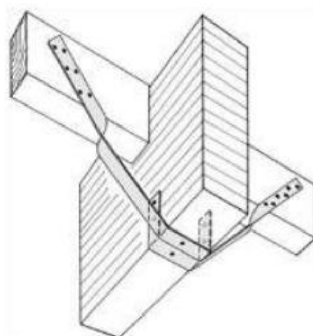
FIGURE 3—TYPICAL TVB KNEE BRACE INSTALLATION
