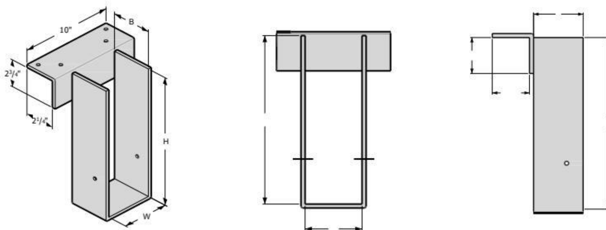
FIGURE 5—TYPICAL TXD SERIES HANGER
