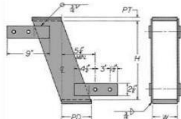
FIGURE 9B—TYPICAL THC HANGER
