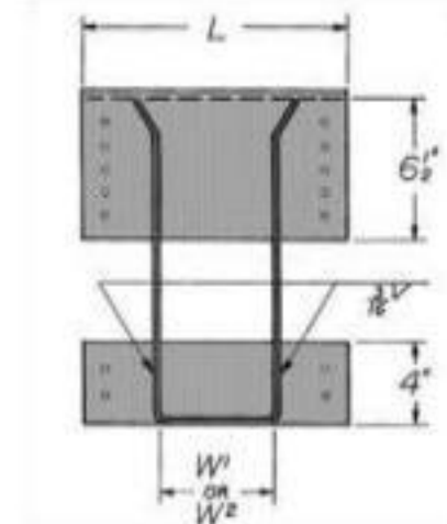
FIGURE 8C—TYPICAL THGLS HANGER
