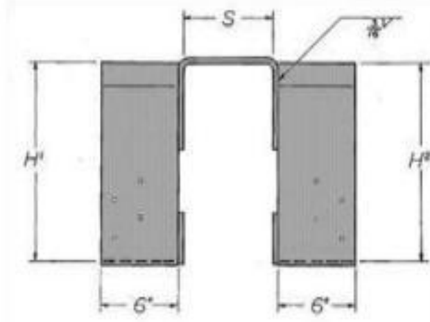
FIGURE 8B—THGLS HANGER
