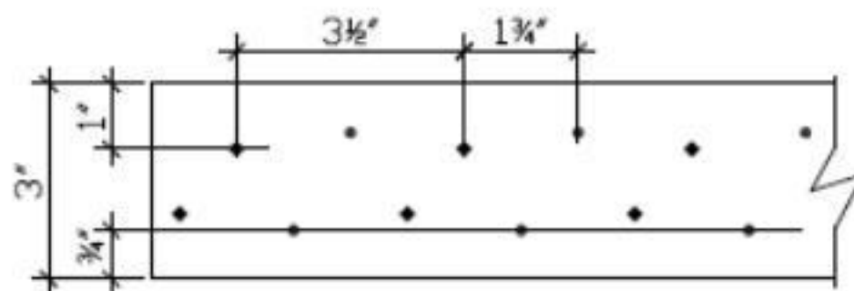
FIGURE 10E—DRAWING OF THE TCMST12 AND TCMST14 STRAPS
