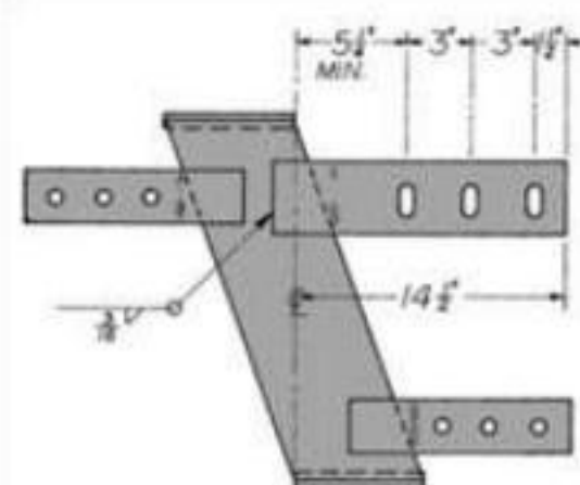
FIGURE 9A—TYPICAL INSTALLATION OF A THC HANGER
