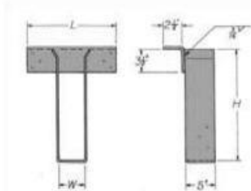
FIGURE 6A—TYPICAL TGLT SERIES HANGER L
