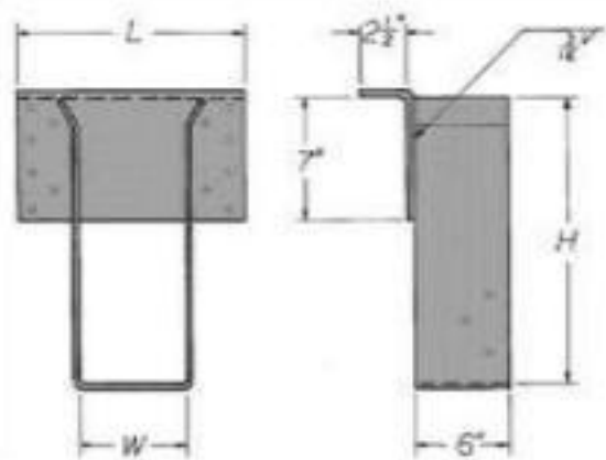
FIGURE 6C—TYPICAL THGLT SERIES HANGER
