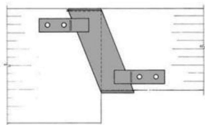
FIGURE 9A—TYPICAL INSTALLATION OF A THC HANGER
