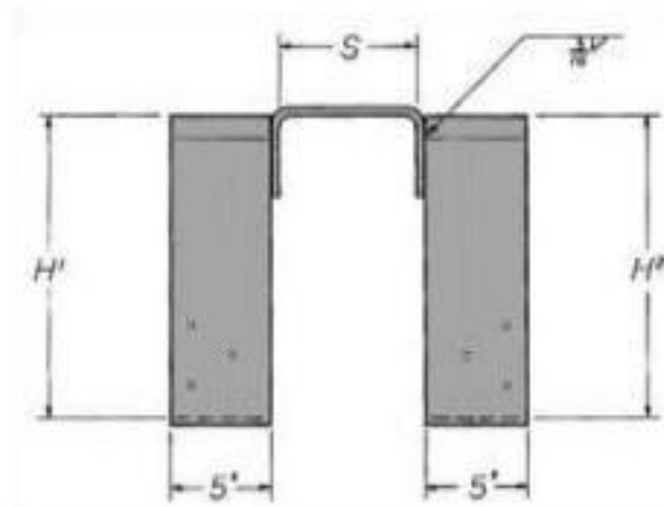
FIGURE 8A—TGLS HANGER
