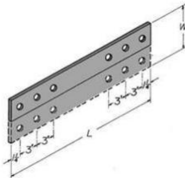
Figure 10B—DRAWING OF THE THST STRAP
