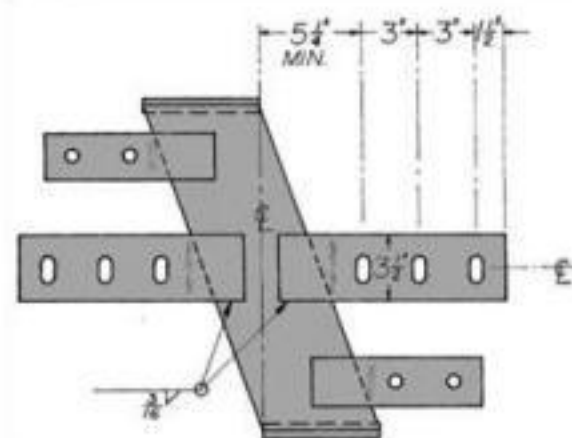
FIGURE 9C—TYPICAL THCCT HANGER
