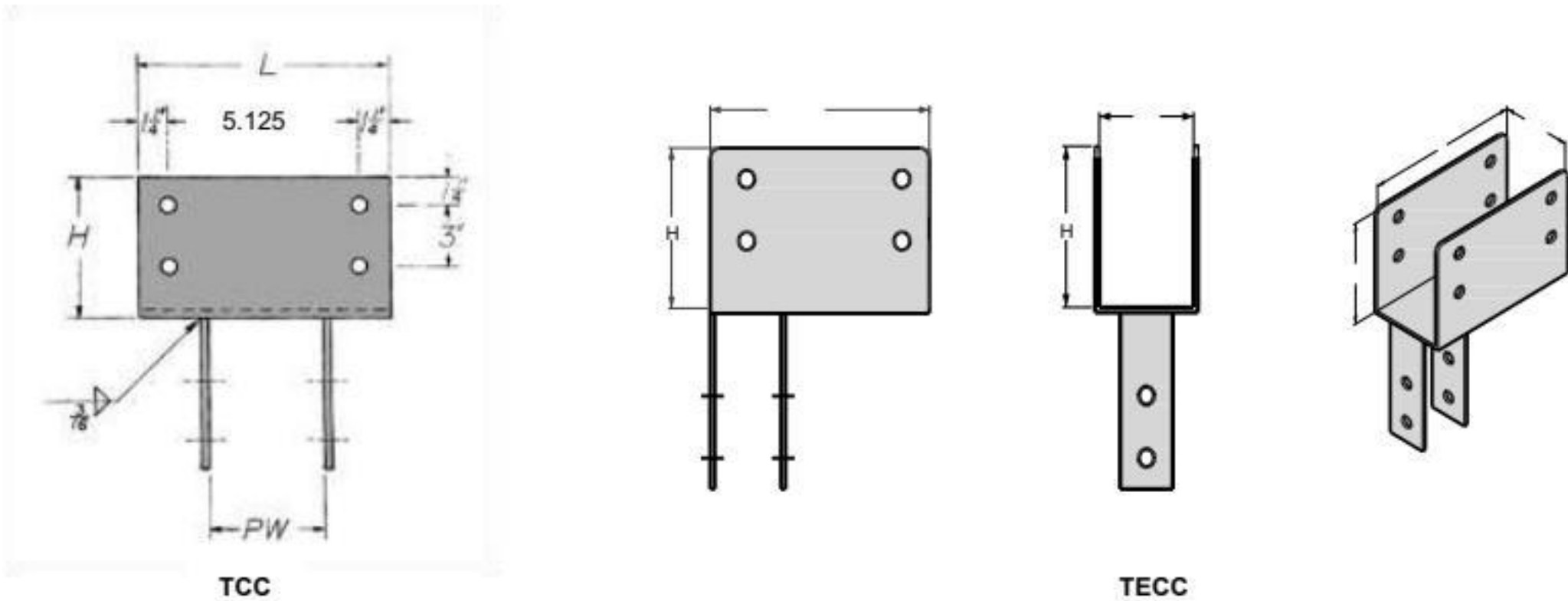
FIGURE 1—TYPICAL TCC and TECC COLUMN CAP CONNECTORS
